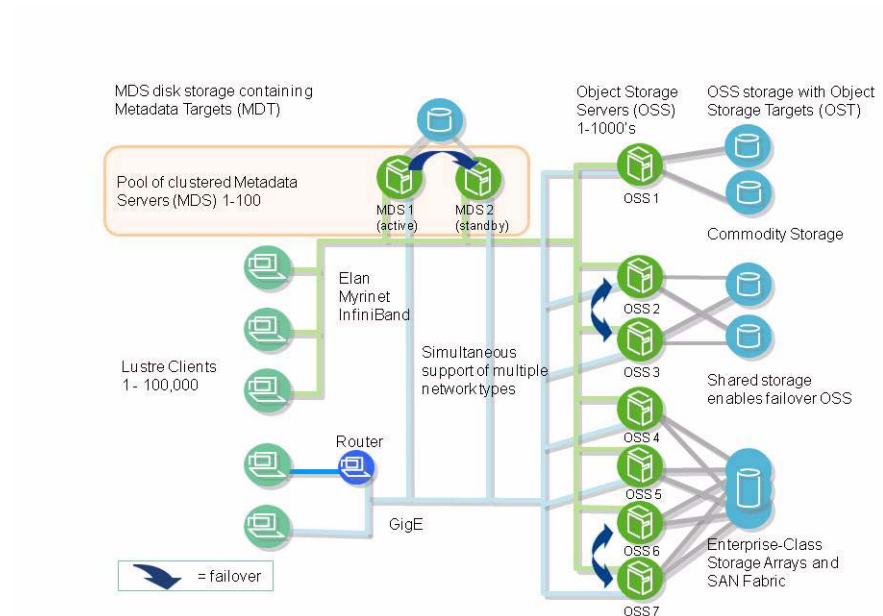
FIGURE 1-3 Lustre cluster at scale
